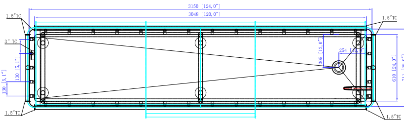
MOTOR MOUNTING PLATE ALL MATERIAL TO BE SS 304
